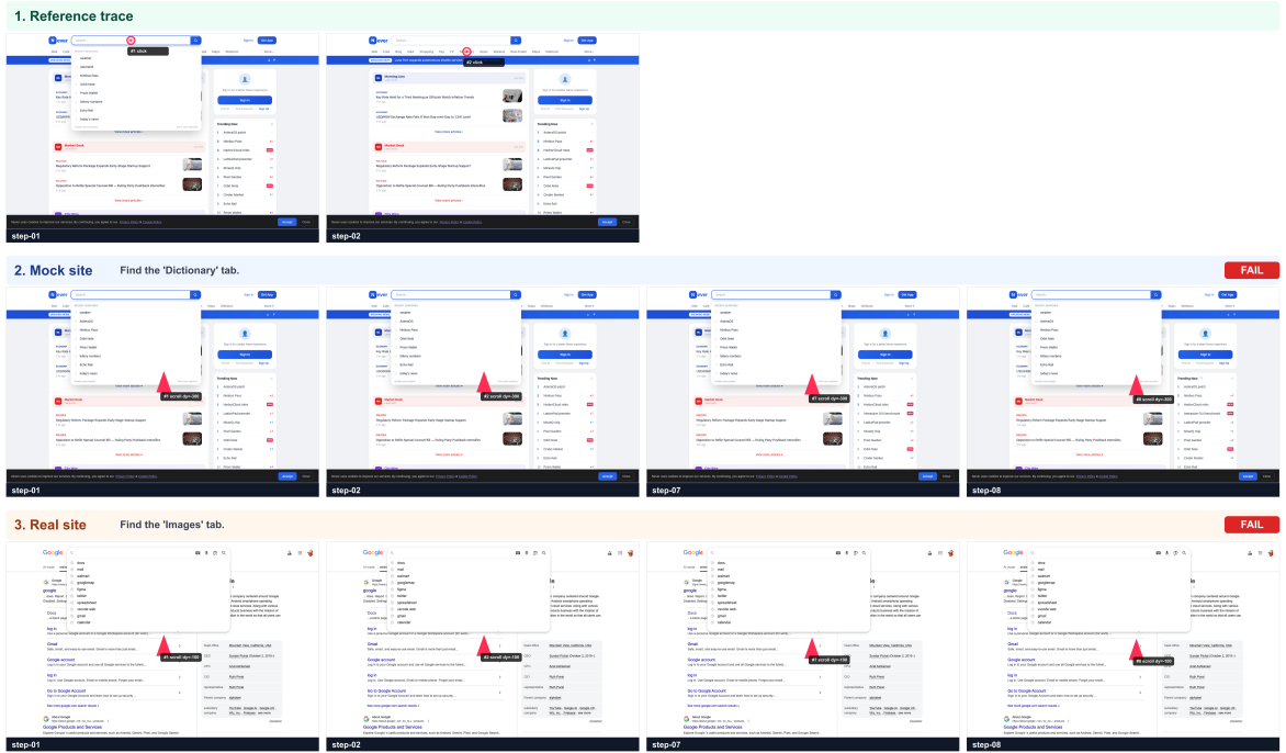
(a) Qwen2.5-VL
