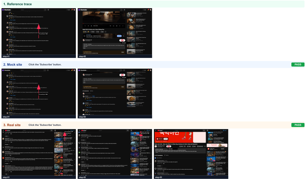
(a) GUI-Owl-1.5
